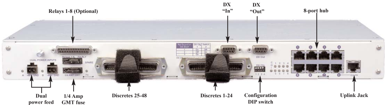
Figure 3 - The back panel offers easy connectorization for power feeds, discrete alarms, relays, and 10BaseT hub.
